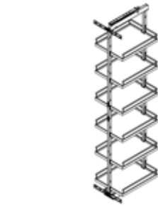
Pull-out for high cabinet / W40 H200 / H220
